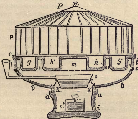
FIG. 38. Lecoq's Propagating-oven.
